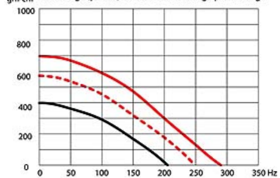
gm-cm Start range (pull-in) with constant voltage power stage
