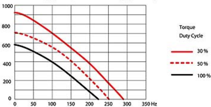
gm-cm Start range (pull-in) with constant voltage power stage
